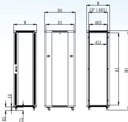
FD1 Rack Size of Standard Model - W600MM
