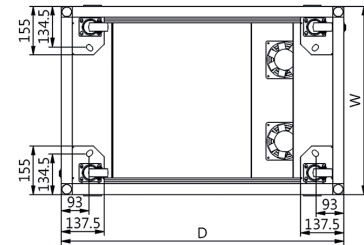
Schematic diagram of the caster bracket
