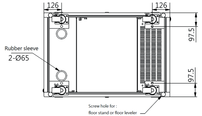
Schematic diagram of the caster bracket
