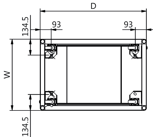
Schematic diagram of the caster bracket
